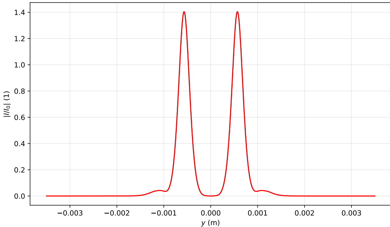
Intensity profile I(x=0, y, z=0.796)/I_0 , \text{Pin}=7.0\text{Pcr} , artificial time
